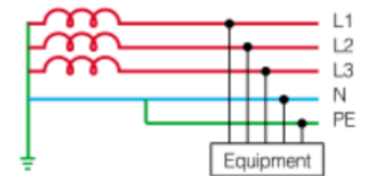
TNC-S system 230/400 V
